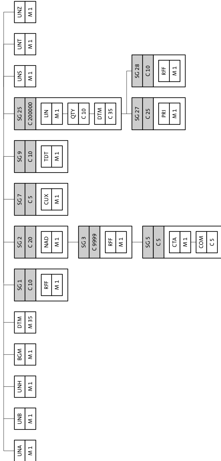
Branching diagram of order response message
